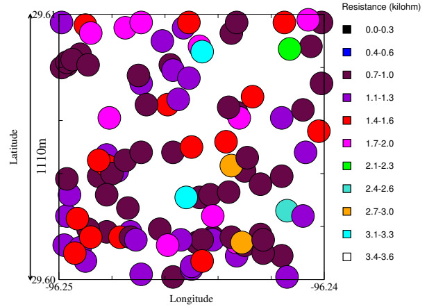
Figure 7: Calculated resistance values ( k\Omega ) plotted on a map.
