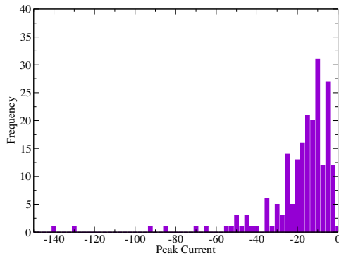
Figure 6: Peak current distribution for 204 negative lightning strikes in an area of about 32,000 m 2 between 2000 and 2011.
