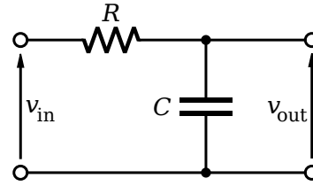
Figure 1: RC circuit
