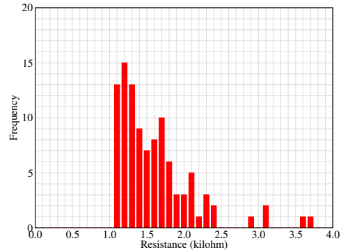
Figure 8: Histogram of resistance values
