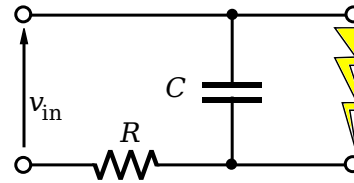
Figure 2: A better approximation of the lightning circuit
