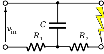
Figure 3: An even better approximation of the lightning circuit
